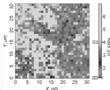
Loss modulus
