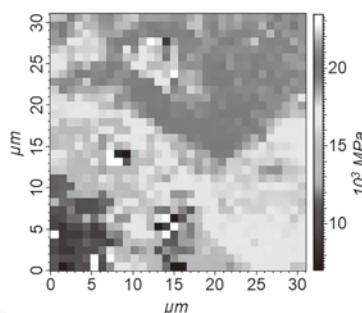
Storage modulus
