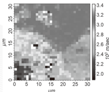
Acoustic speed
